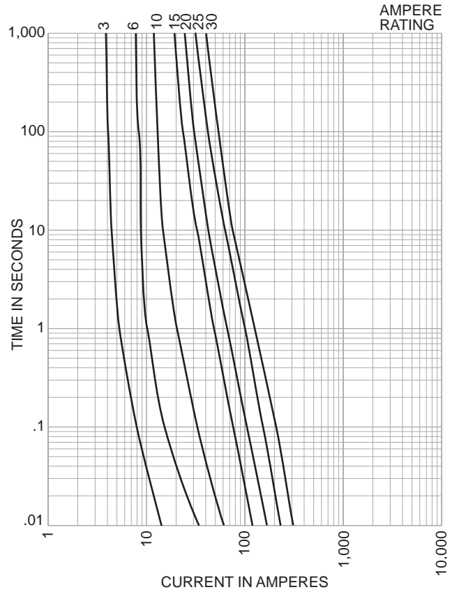
Time/Current-Curves (Cat. No. CIF06)
